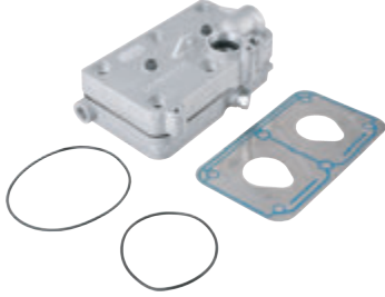
Silindir Kapak Komple Cylinder Head Complete 20701803-412 704 932 2
