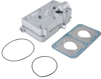
Silindir Kapak Komple Cylinder Head Complete 412 704 925 2
