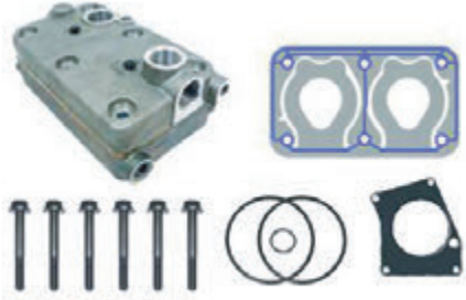
Silindir Kapak Komple Cylinder Head Complete 911 553 001 2 - 001 130 0815
