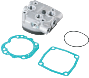
Silindir Kapak Komple Cylinder Head Complete 447 130 0019
