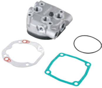
Silindir Kapak Komple Cylinder Head Complete 447 130 0019
